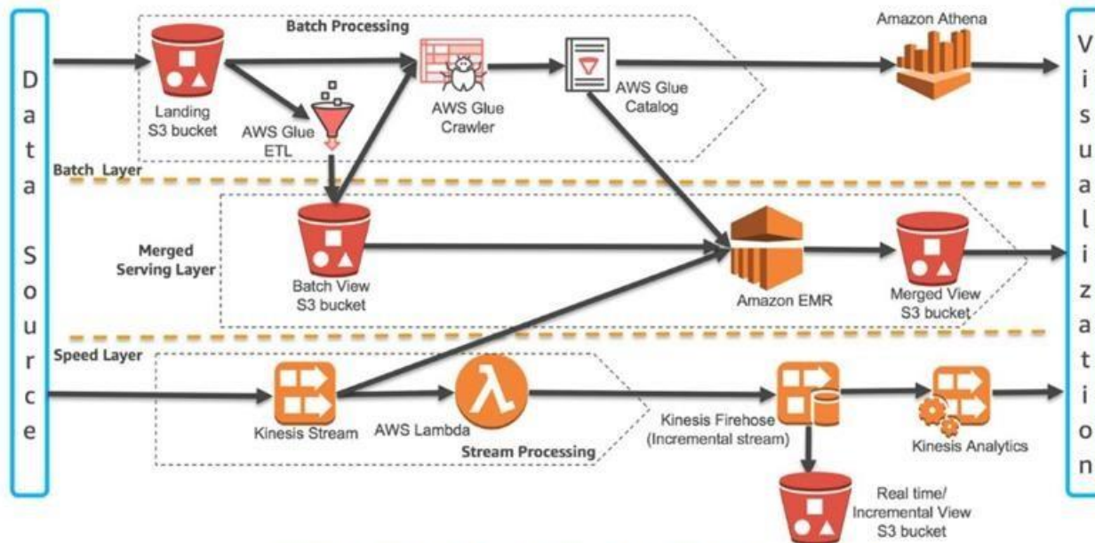
Figure 2: Lambda Architecture Building Blocks on AWS
