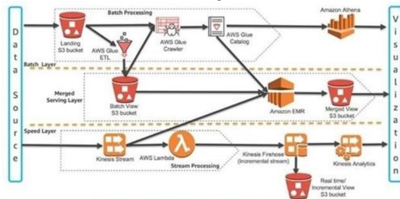
Figure 2: Lambda Architecture Building Blocks on AWS
